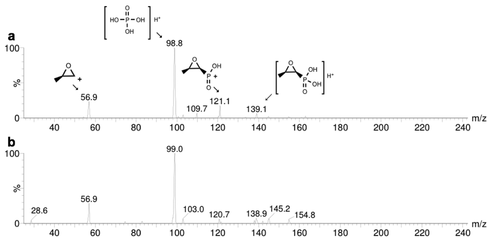
Figure 3. MS/MS fragmentation of the ammonium form of fosfomycin phosphate (mass of 236) produced by THA IPK and S. wedmorensis FomA. (a) Fragmentation of the product formed by THA IPK showed peaks corresponding to [\text{C}_3\text{H}_5\text{O}]^+ (mass of 56.9), [\text{H}_4\text{O}_4\text{P}]^+ (mass of 98.8), [\text{C}_3\text{H}_6\text{O}_3\text{P}]^+ (mass of 121.1), and [\text{C}_3\text{H}_8\text{O}_4\text{P}]^+ (mass of 139.1). The same peaks were found in the fragmentation product formed by S. wedmorensis FomA (b).
